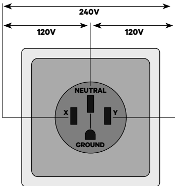
14-50R 240V/50A "RV" outlet
